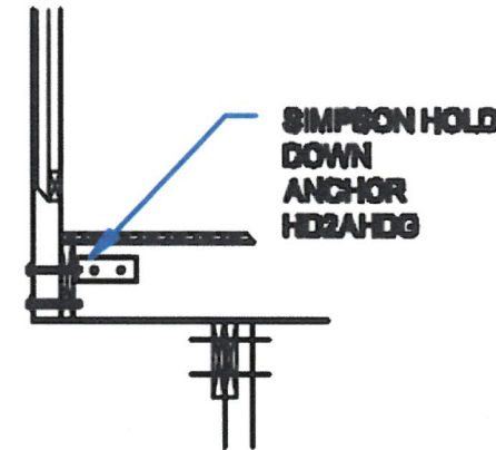
GUARD POST MOUNTED ON OUTSIDE OF RIM BOARD PERPENDICULAR TO JOIST
