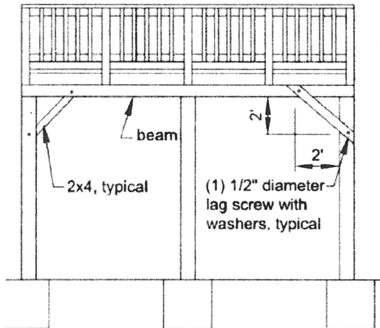
GUARD POST CONNECTION TO RIM BOARD
