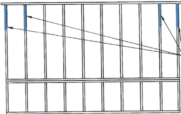
EXTERIOR TENSION-TIE LOCATIONS (4 total)
