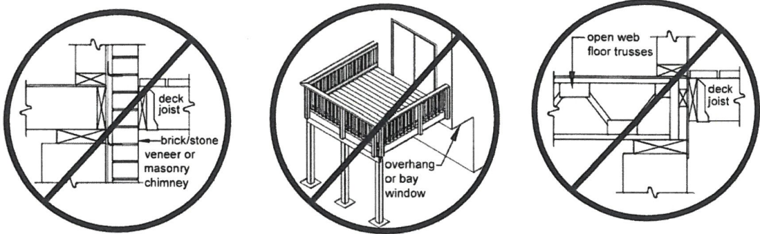
PROHIBITED CONNECTIONS
